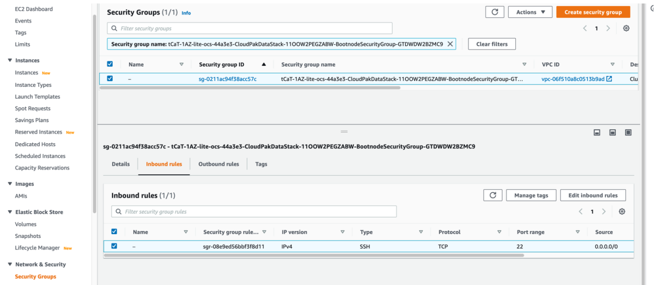
Figure 11: Security Groups
