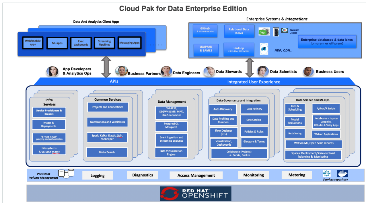
Figure 3: Software Hub services
